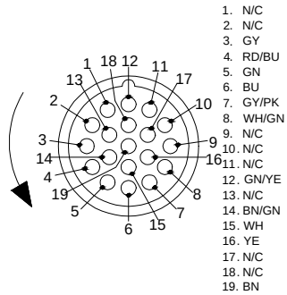
FEMALE END VIEW
